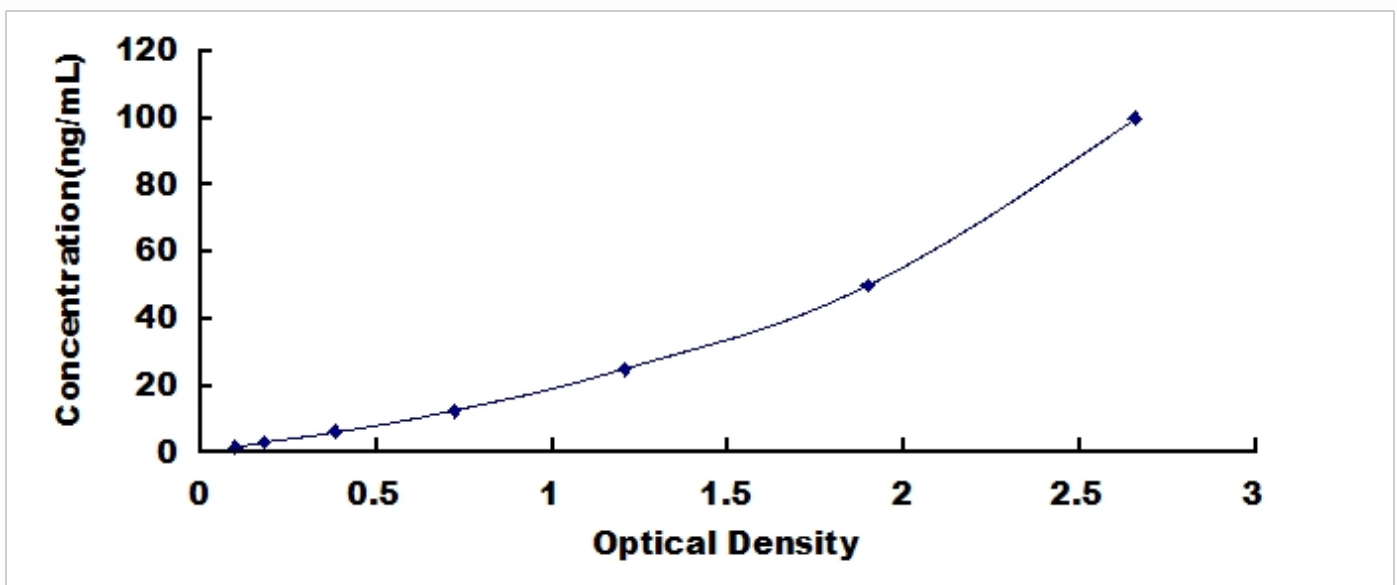
Typical Standard Curve for NGAL, Rabbit ELISA.
